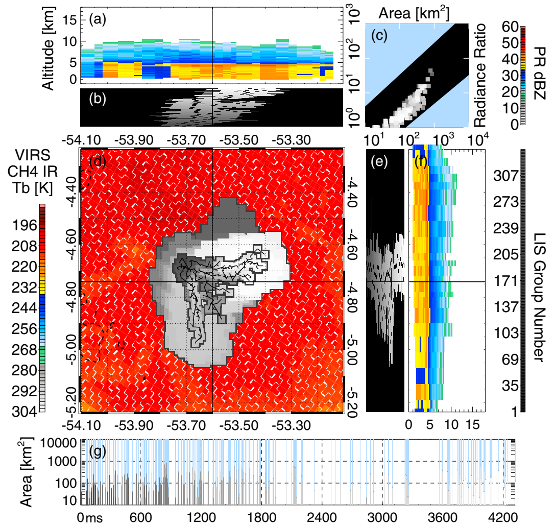
Figure 8. The same as Figure 1 for the longest-lasting entirety stratiform propagating LIS flash.
