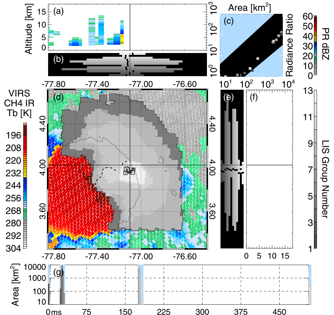
Figure 4. The same as Figure 1 for the LIS flash with the largest separation of events.
