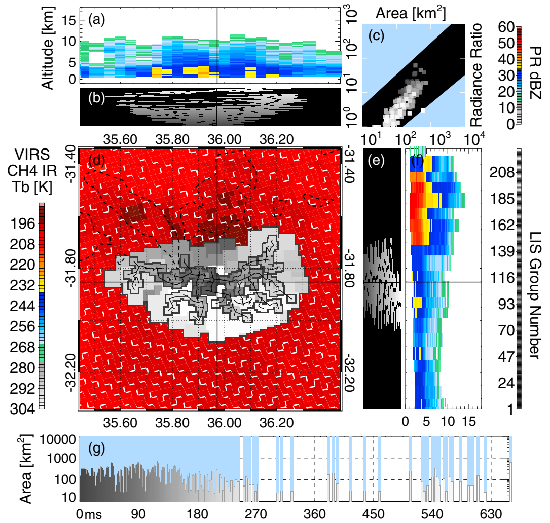
Figure 9. The same as Figure 1 for the LIS flash with the longest-lasting series.
