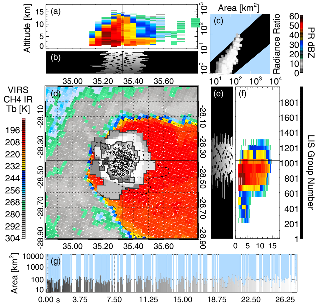
Figure 6. The same as Figure 1 for the LIS flash with the most bright series.
