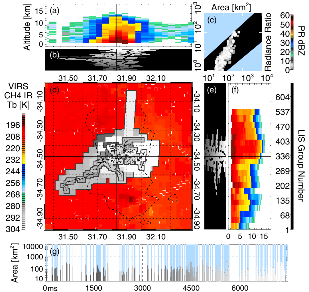
Figure 7. The same as Figure 1 for the longest-lasting convective-to-stratiform propagating LIS flash.
