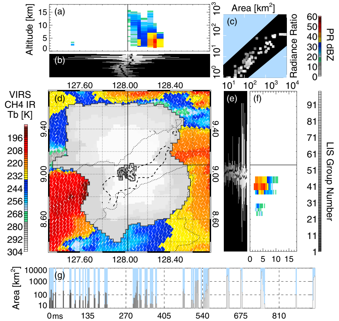
Figure 3. The same as Figure 1 for the LIS flash with the largest footprint area.
