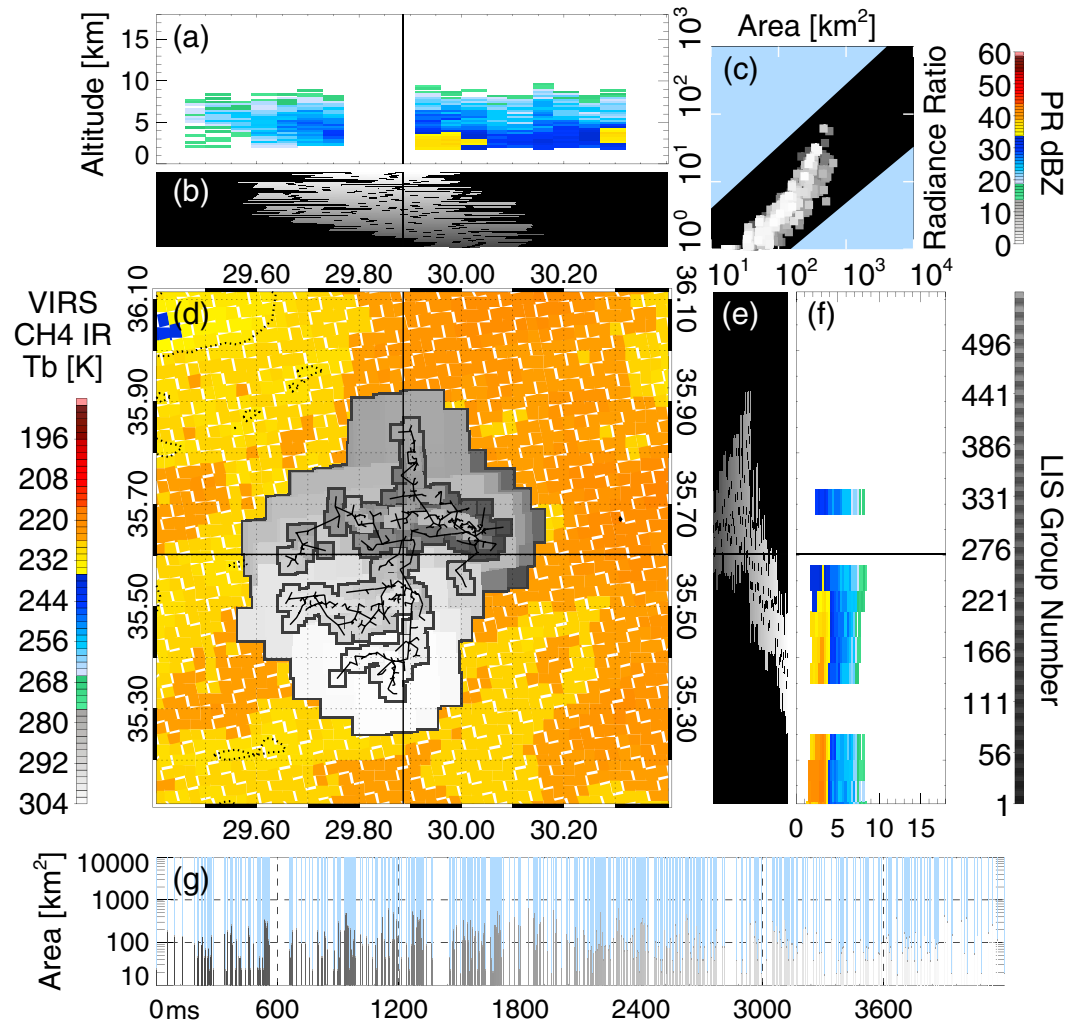
Figure 2. The same as Figure 1 for the LIS flash with the most visible branches.
