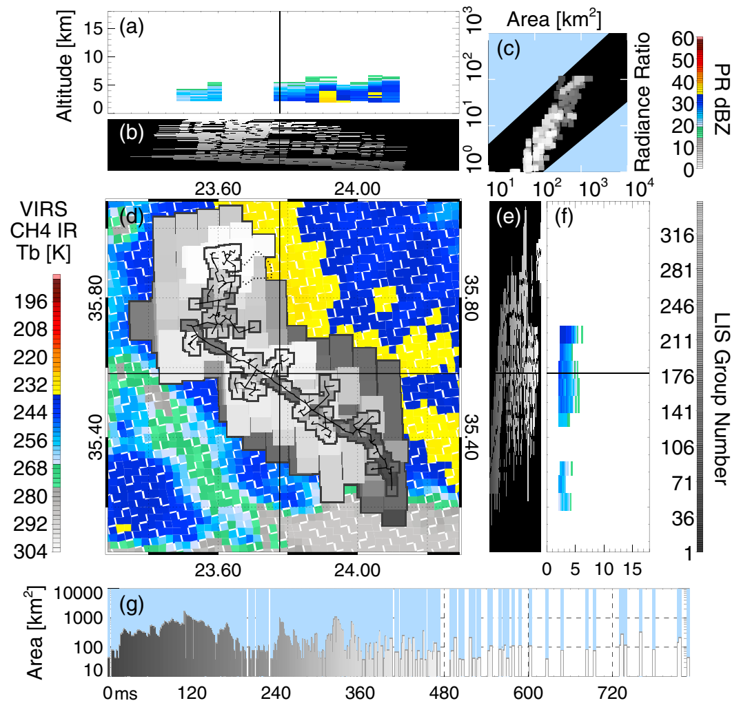
Figure 1. The LIS flash with the largest separation of groups. LIS events (large pixels) and group centroids (small boxes) are coded by LIS group number. (a) PR reflectivity longitude-altitude cross section. (b) Longitude extent of LIS groups. (c) Radiance-area profile of LIS groups in the flash (approximate boundaries from Peterson et al., 2016 shaded blue). (d) Plan view on top of VIRS CH4 10.8 μm brightness temperatures (colored pixels). PR convective features (dashed lines) and VIRS CH4 <225 K regions (dotted lines) are shaded. (e) Latitude extent of LIS groups. (f) PR reflectivity latitude-altitude cross section. (g) Time series of LIS groups (greyscale) and series (blue shaded).
