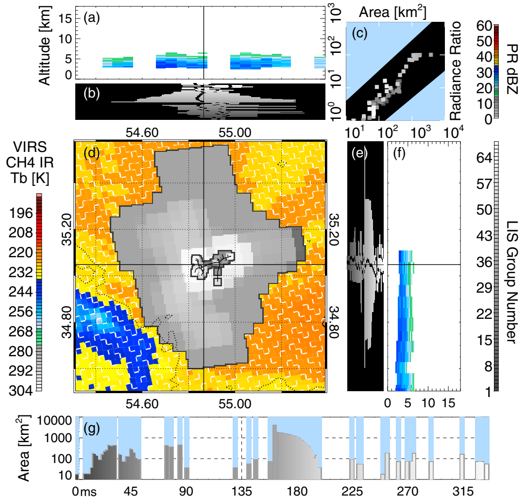
Figure 5. The same as Figure 1 for the LIS flash with the most radiant group.
